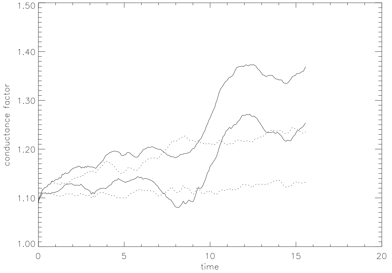
Conductance Correction to MHD – North
